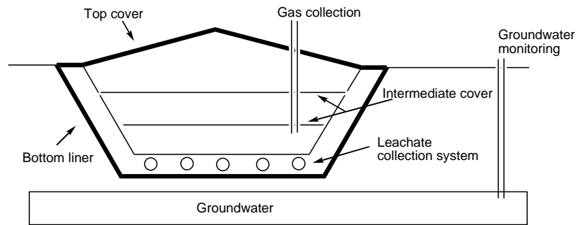
Figure 11: Construction of a modern landfill.
