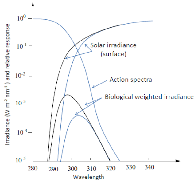
Figure 15: Biological weighted irradiance combining action spectra with solar irradiance. The blue curves indicate irradiance under normal ozone condition while black line corresponds to a reduction in ozone. (Source: Ref. 1)
