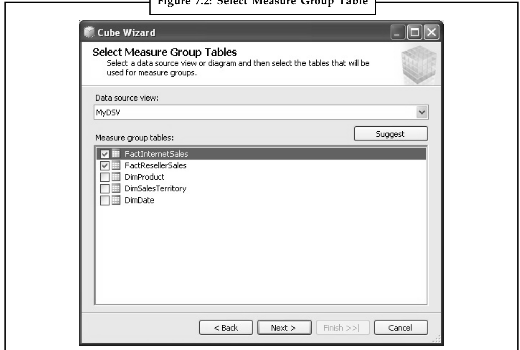
Figure 7.2: Select Measure Group Table
