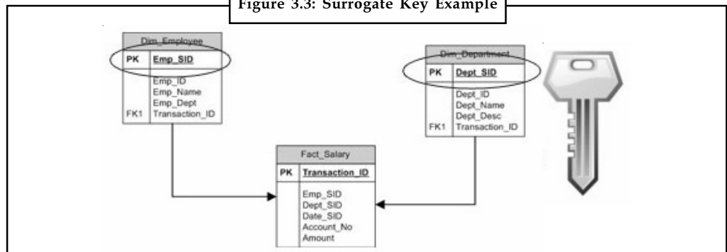
Figure 3.3: Surrogate Key Example
