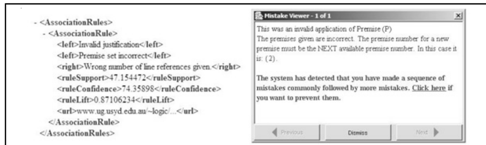
(a) XML encoded patterns
