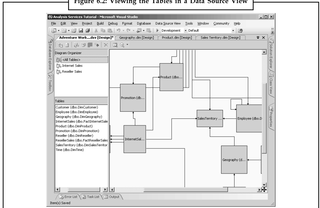
Figure 6.2: Viewing the Tables in a Data Source View
