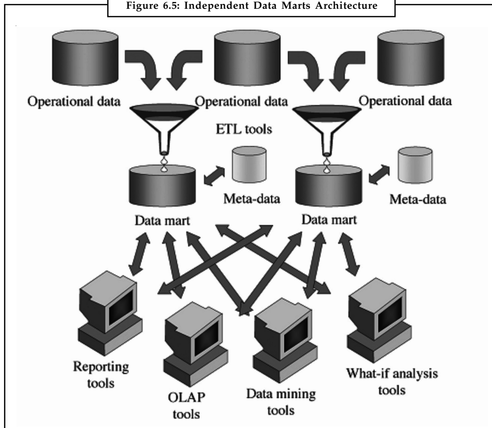
Figure 6.5: Independent Data Marts Architecture
