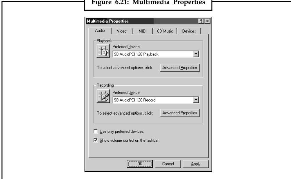
Figure 6.21: Multimedia Properties
