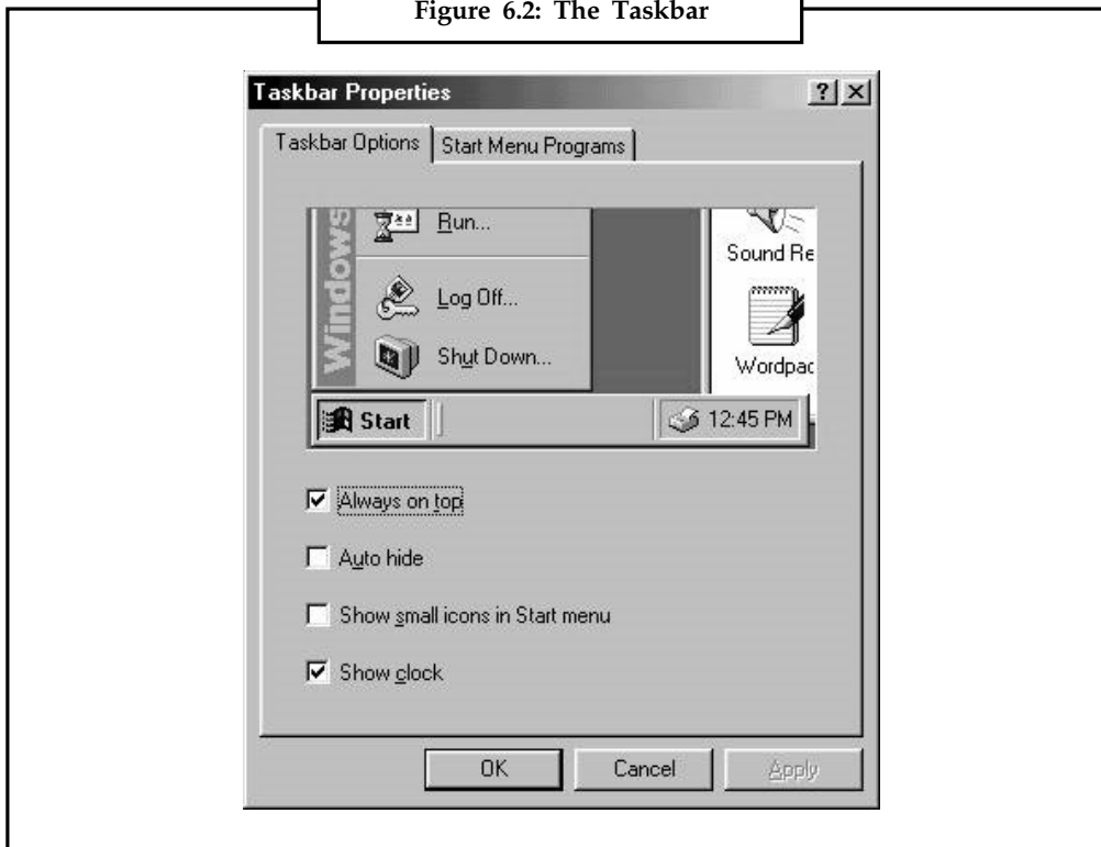
Figure 6.2: The Taskbar
