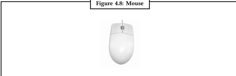
Figure 4.8: Mouse
