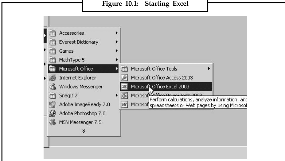
Figure 10.1: Starting Excel
