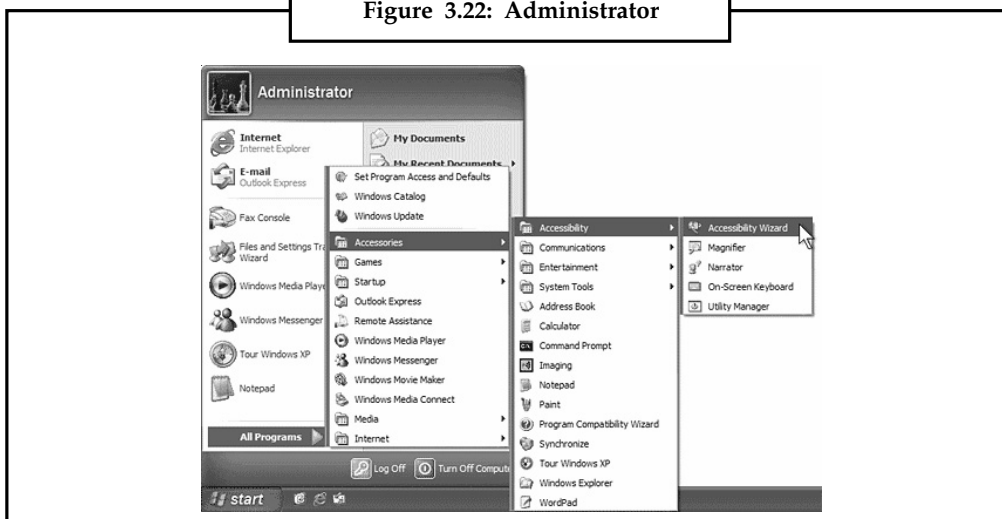
Figure 3.22: Administrator
